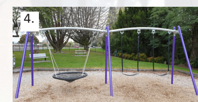
4. triple swing frame
